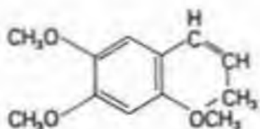
1, 2, 4-TRIMETHOXY-5-PROPENYLBENZENE (ASARONE)
